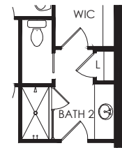
Shower @ Bath 2
